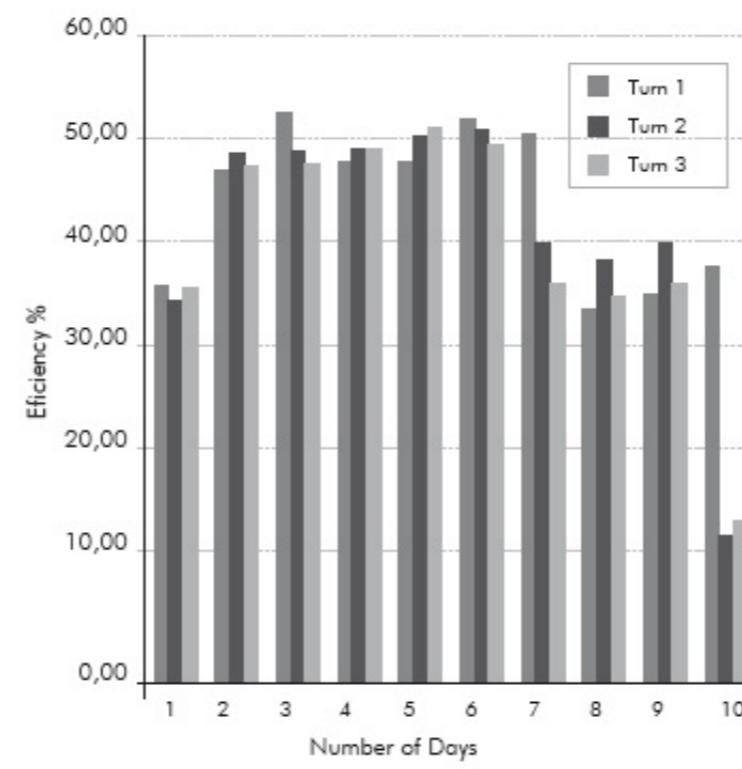
Figure 8. Thermal Efficiency of HRSGs by the direct method.
